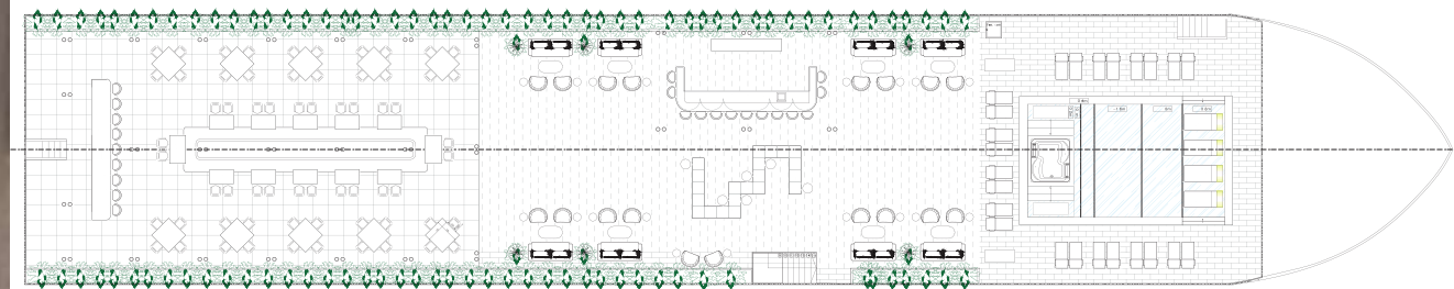
SUNDECK PLAN
